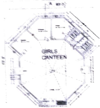
PLAN (BLOCK 13)
